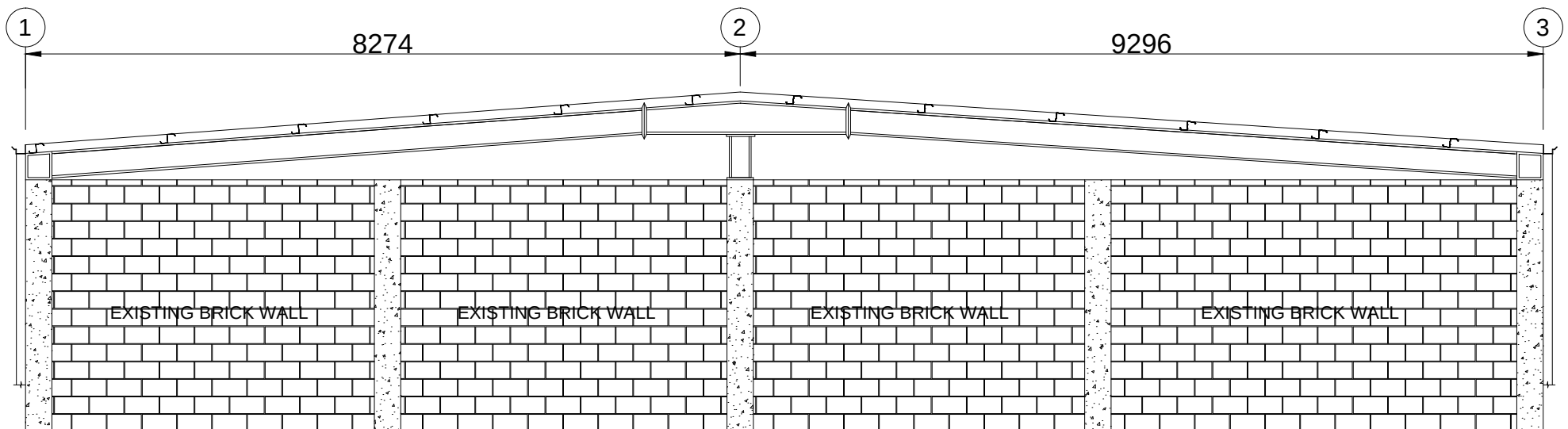
CROSS SECTION GRID-A
